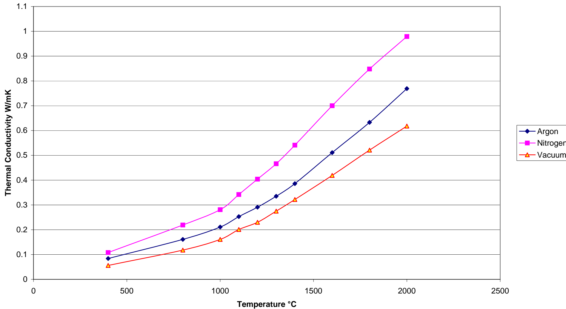
Thermal Conductivity of Virgin Fibre CBCF Board
