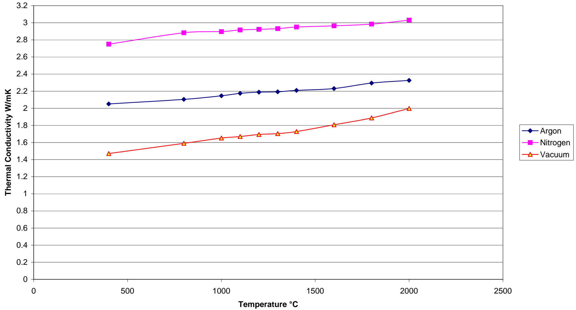
Thermal Conductivity of High Density CBCF Board
